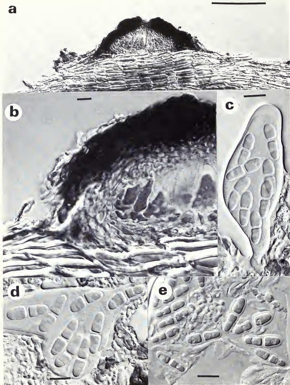
Fig. 25 Arthopyrenia stenospora Körber (L-syntype) (a) Vertical section of ascoma; scale = 100 \mu\text{m} ; (b) Detail of involucrellum and exciple showing pseudoparenchymatic tissue of leptodermatous cells; (c) Ascus and ascospores; (d), (e) Ascospores; scale = 10 \mu\text{m} .
